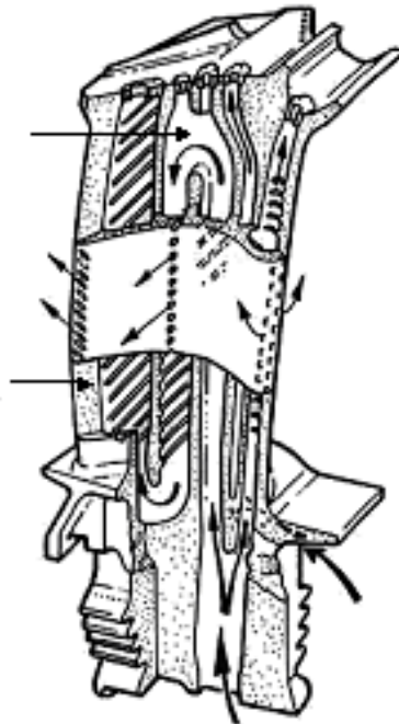
Figure 1. Airflow through a cooled turbine blade (from Rolls Royce, 2005)
